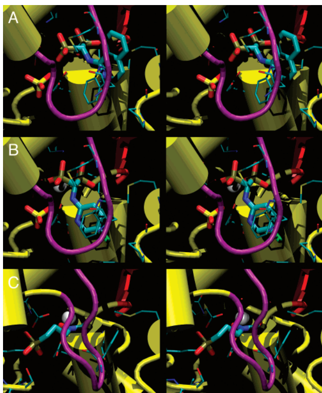
Figure 2. Stereo representations of the catalytic patch of DXR with three inhibitors. A , 2 (PDB file 1T1R); B , 3 (PDB file 1T1S), and C , fosmidomycin (from PDB file 1ONP). The inhibitor side chains are shown in cyan, the sulfate ions (in A and B ) in yellow/red, Mg^{2+} in gray.
