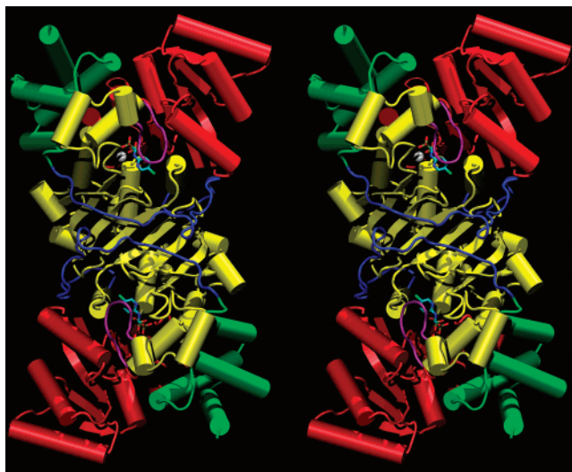
Figure 1. Stereo representation of the overall structure of the complex between 3 and DXR (dimer structure), PDB file 1T1S. The NADP domain is shown in red, the catalytic domain in yellow, the active site loop in purple, and the C-terminal domain in green. The inhibitor 3 is shown in cyan and Mg^{2+} in gray.
